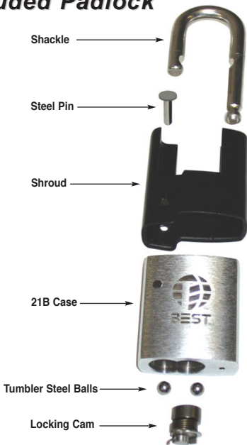
Exploded View 21B Shrouded Padlock
